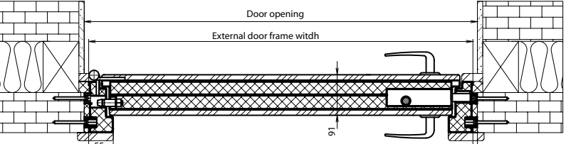
Outer Wall fixing
