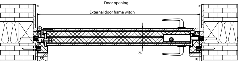
Centred Wall fixing
