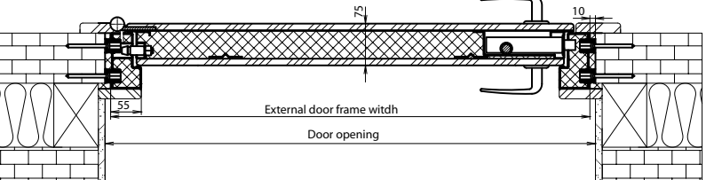
Inner Wall fixing
