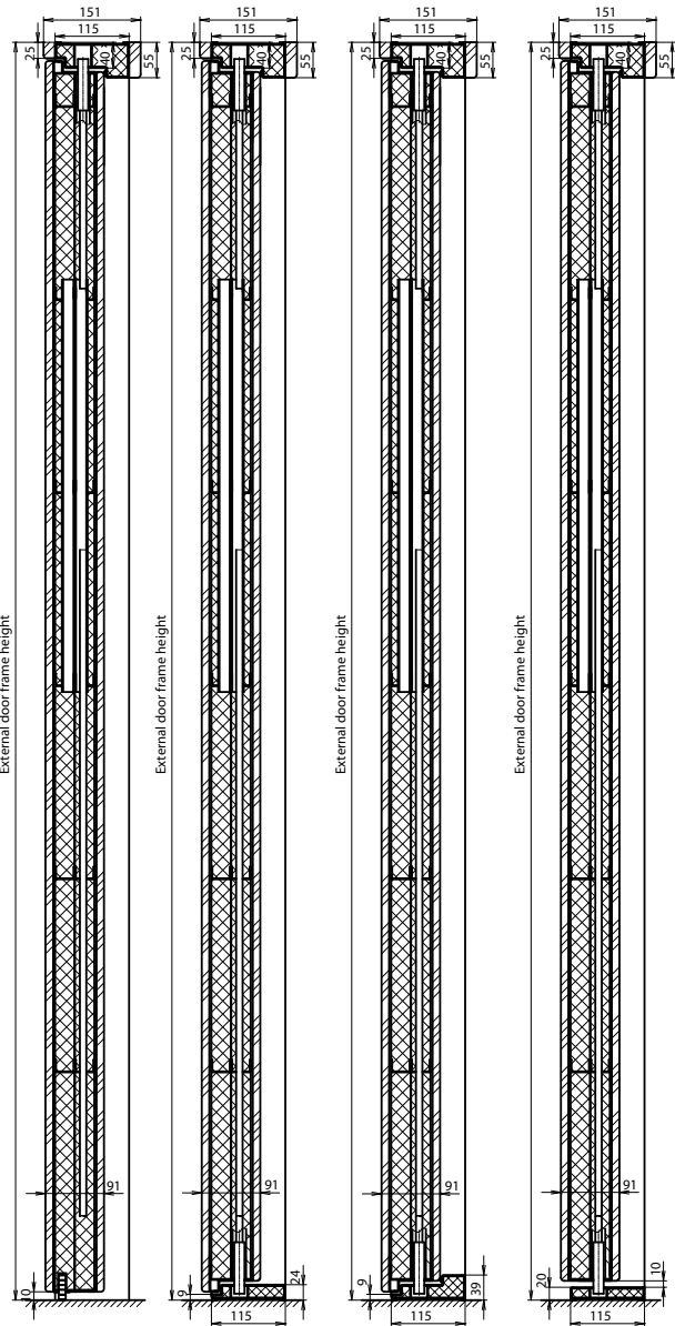
Sliding seal, no step. Flat 24mm x 115mm step. Angled 39mm x 115mm step. Flat 20mm x 115mm step.
