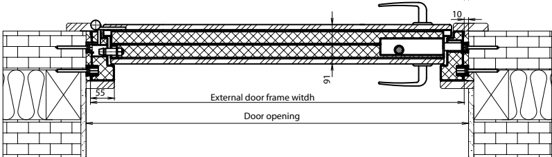
Inner Wall fixing
