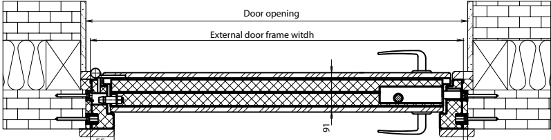
Outer Wall fixing
