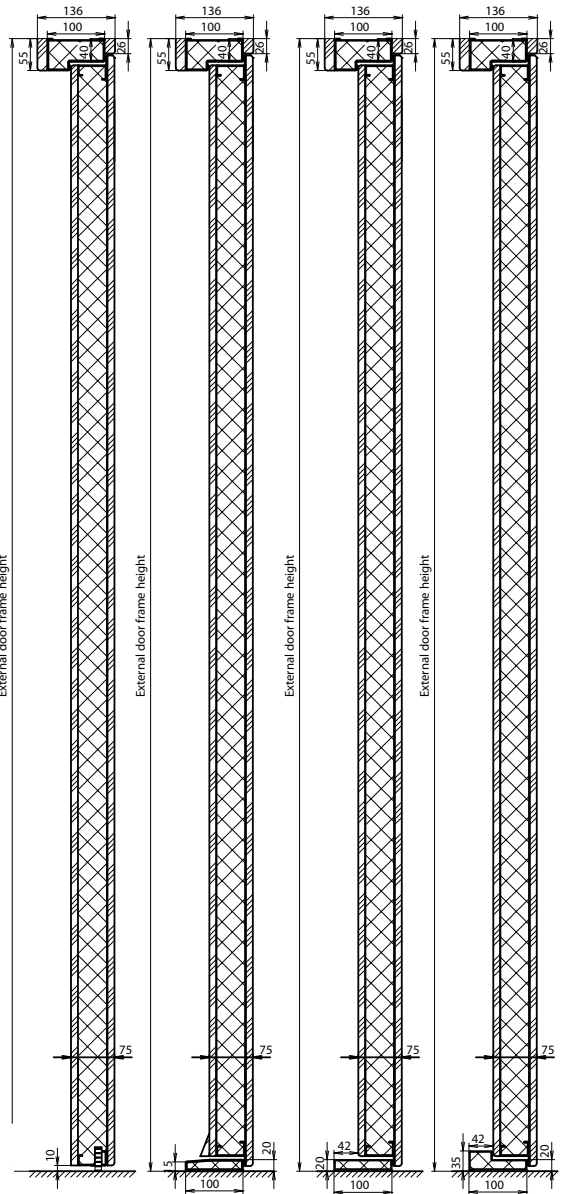
Sliding seal, no step. Flat 24mm x 115mm step. Angled 39mm x 115mm step. Flat 20mm x 115mm step.
