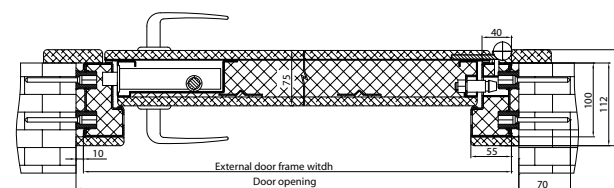
The horizontal cut of fitted door
