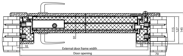
The horizontal cut of fitted door
